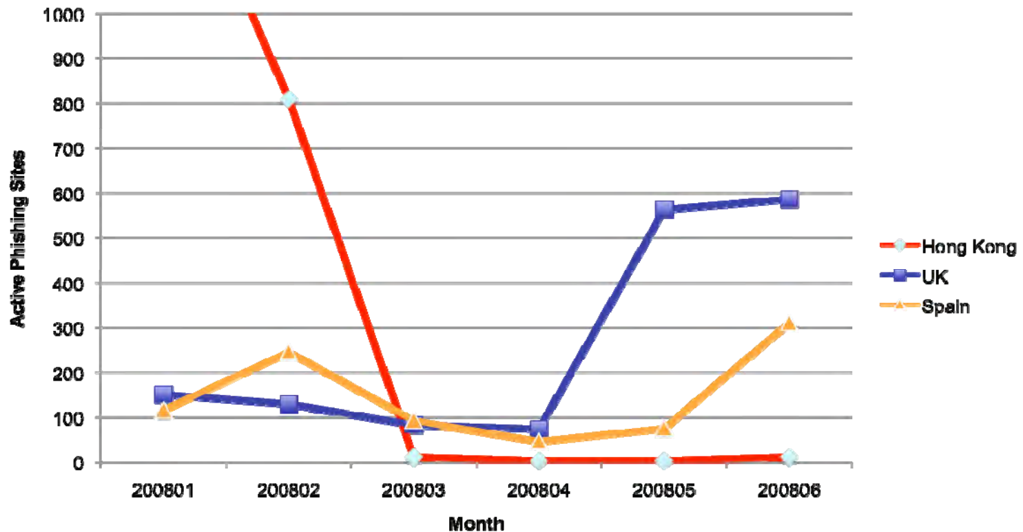
Phishing attacks - Select TLDs targeted by ROCK Phish
