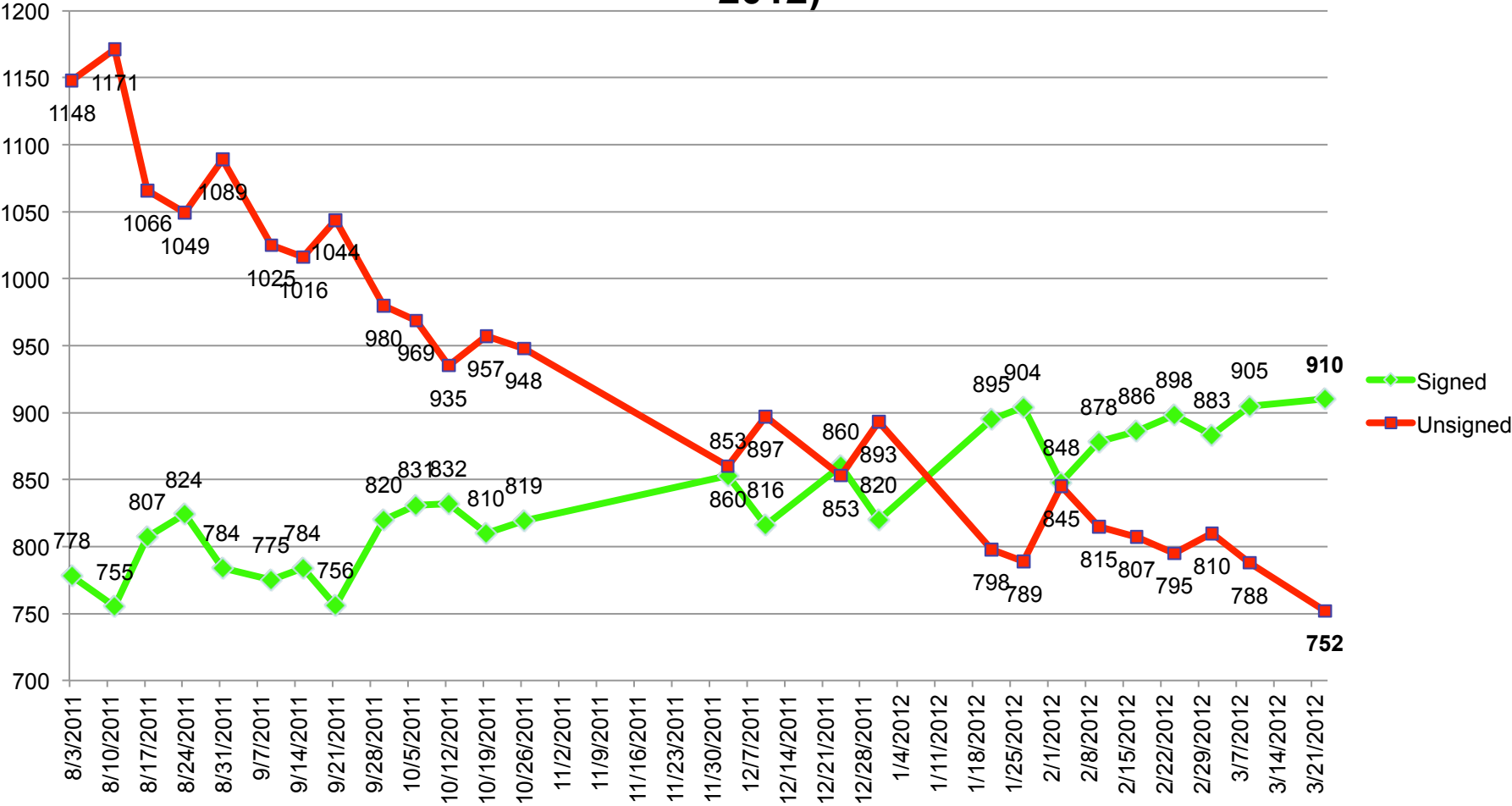
DNSSEC Compliance Trend for all Federal .GOV Domains (August 2011 – March 2012)
