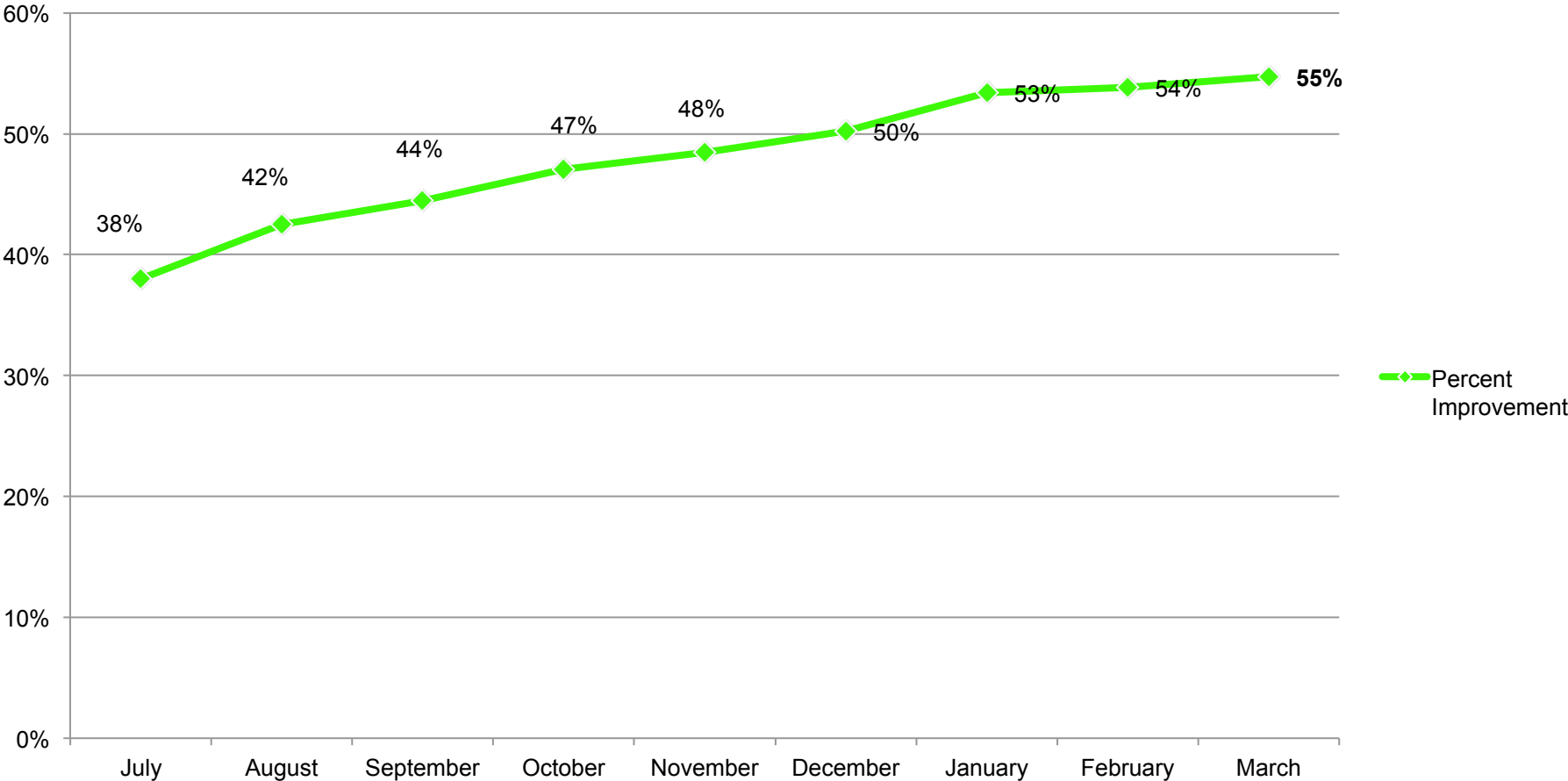
DNSSEC Improvement Trend (July 2011- March 2012) Number of Compliant vs. Total Number of Domains
