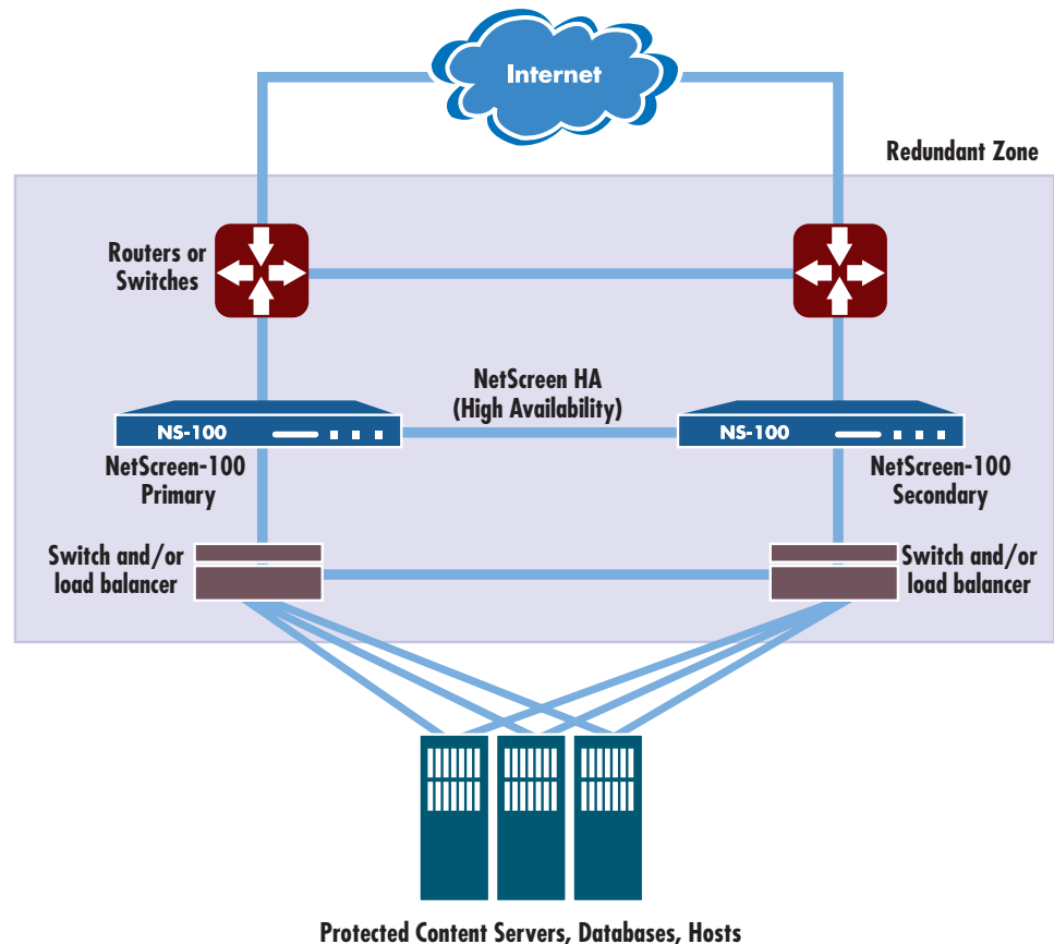
High Availability ensures that data continues to flow to servers should any link or service fail in the "redundant zone."
